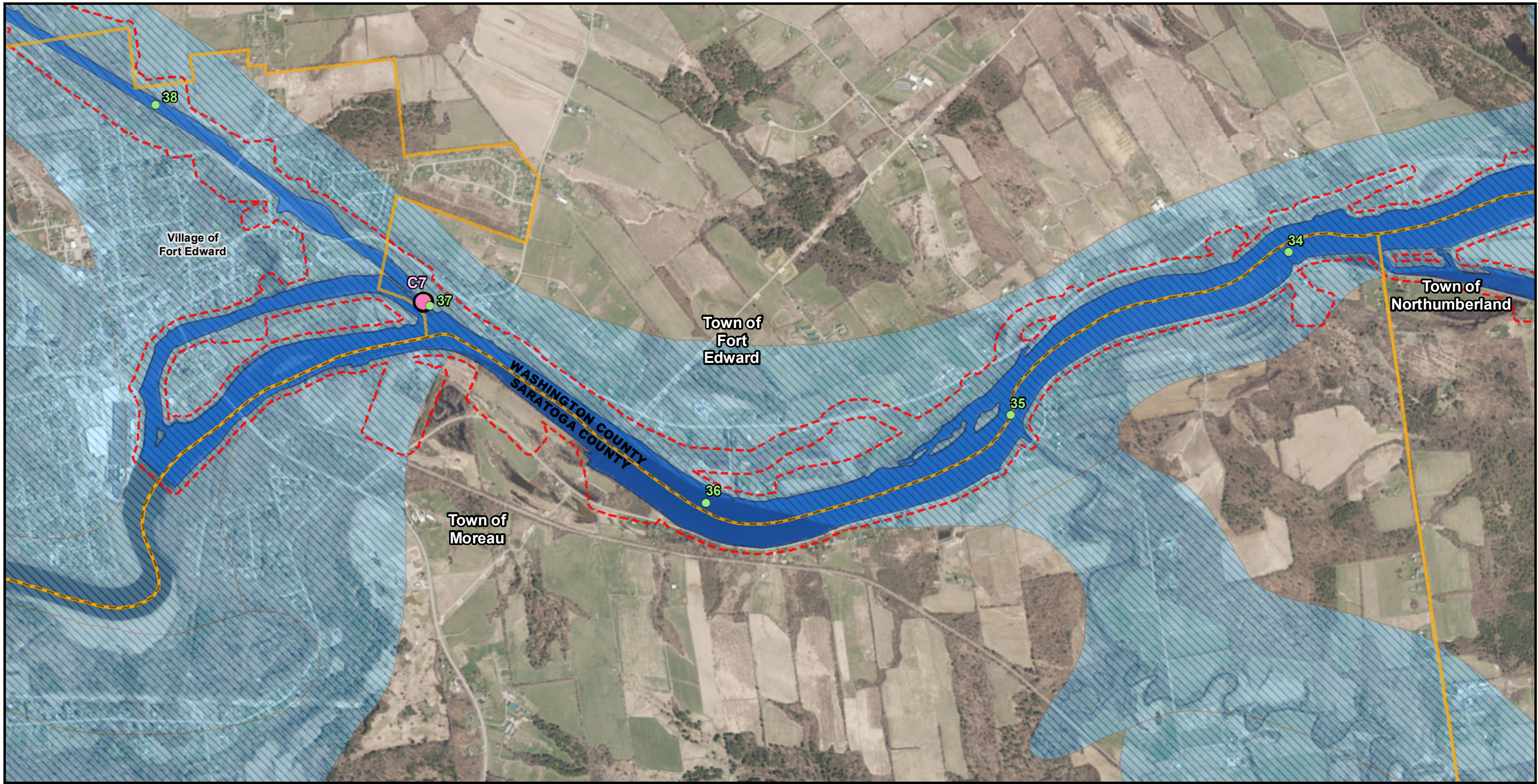
Figure 8F: Aquifers
